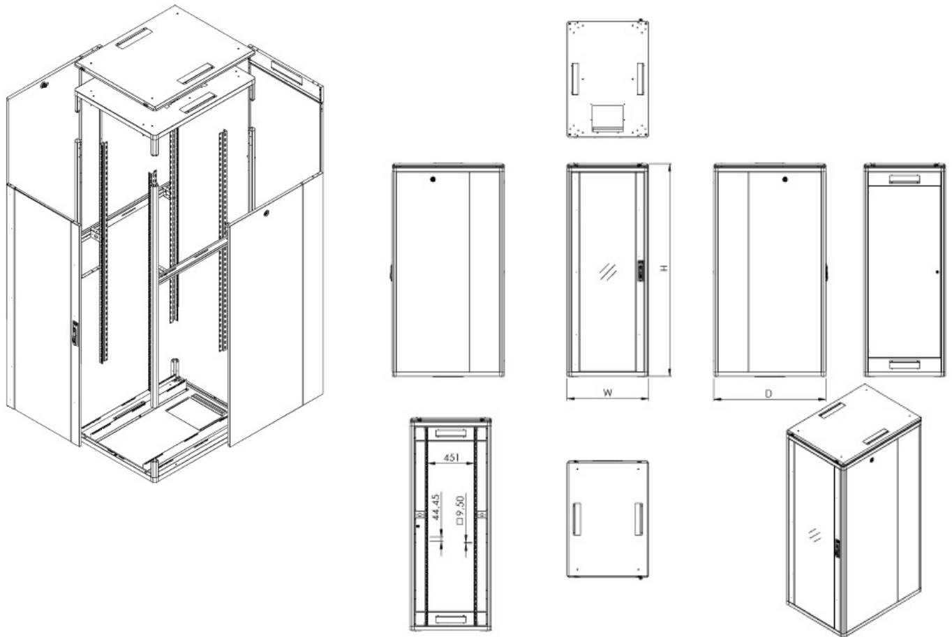
19" Atlas BASIC Free Standing Cabinets W=800 D=1000
