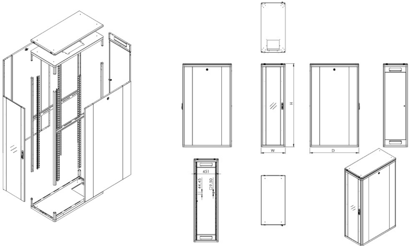
19" Atlas BASIC Free Standing Cabinets W=600 D=1200
