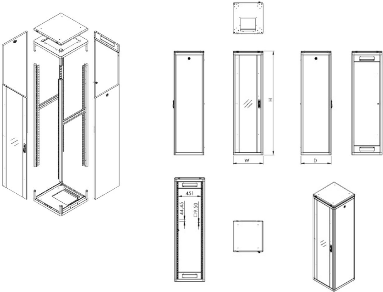
19" Atlas BASIC Free Standing Cabinets W=600 D=600
