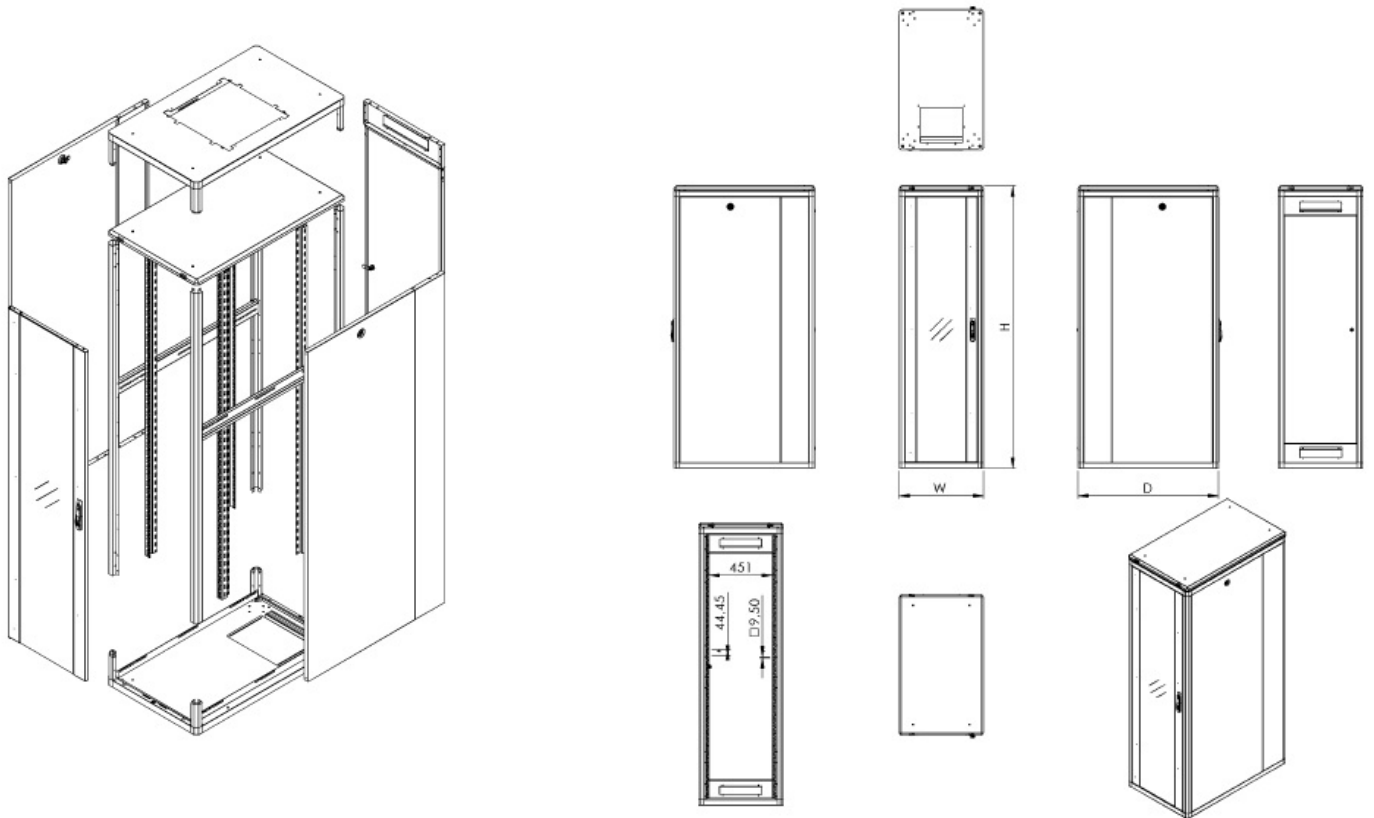
19" Atlas BASIC Free Standing Cabinets W=600 D=1000
